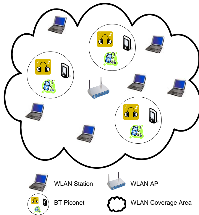
Fig. 1. Network topology of spatially overlapped BT piconets and WLAN stations within a WLAN's coverage area. The WLAN's topology could be infrastructure-based (as shown) or based on the ad hoc mode.
