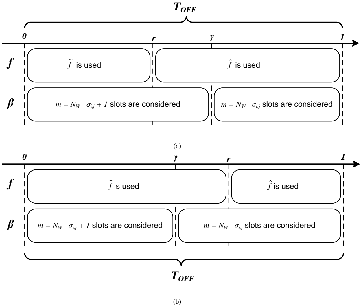
Fig. 5. The dependence of f and \beta on the length of T_{OFF} for (a) ( r \leq \gamma ), and (b) ( r > \gamma ).
