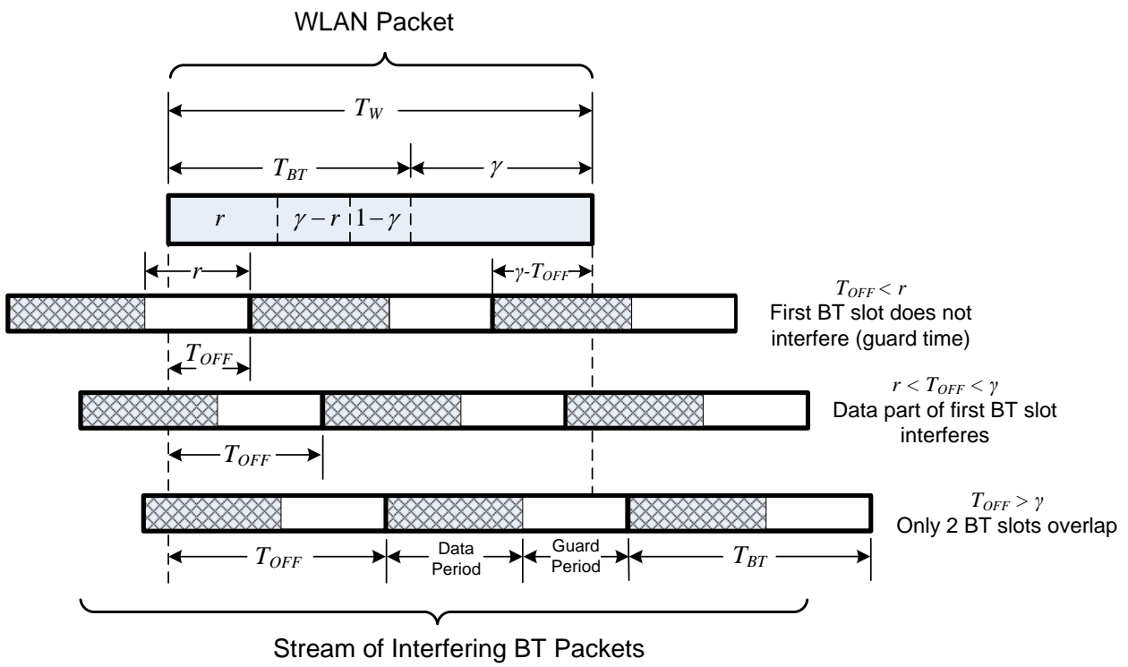
Fig. 4. Temporal overlappings of simultaneously transmitted WLAN and BT packets for the case ( T_W > T_{BT} ) and ( r \leq \gamma ).
