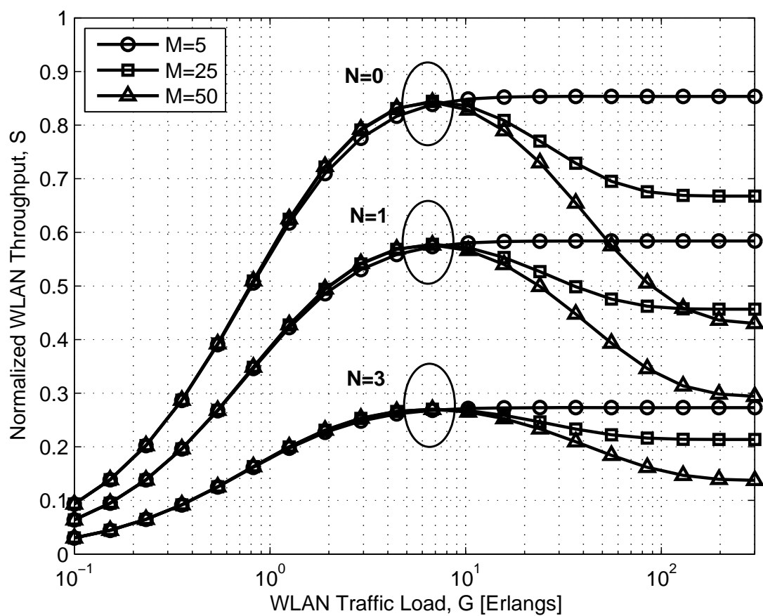
Fig. 9. CSMA throughput as a function of its offered traffic load G , WLAN packet size = 1400 bytes ( T_W = 1193 \mu s ), p = 0.03 , 60% piconet traffic ( \rho_0 = 0.4 ), and equal arrivals of DH1/3/5 ( \rho_1 = \rho_3 = \rho_5 ).
