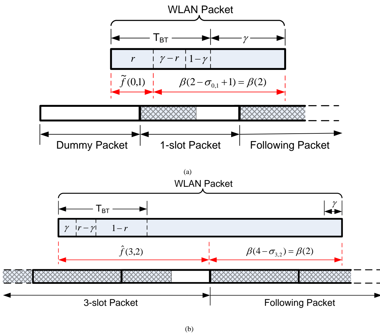
Fig. 6. Examples of success probability calculations for different WLAN packet lengths.
