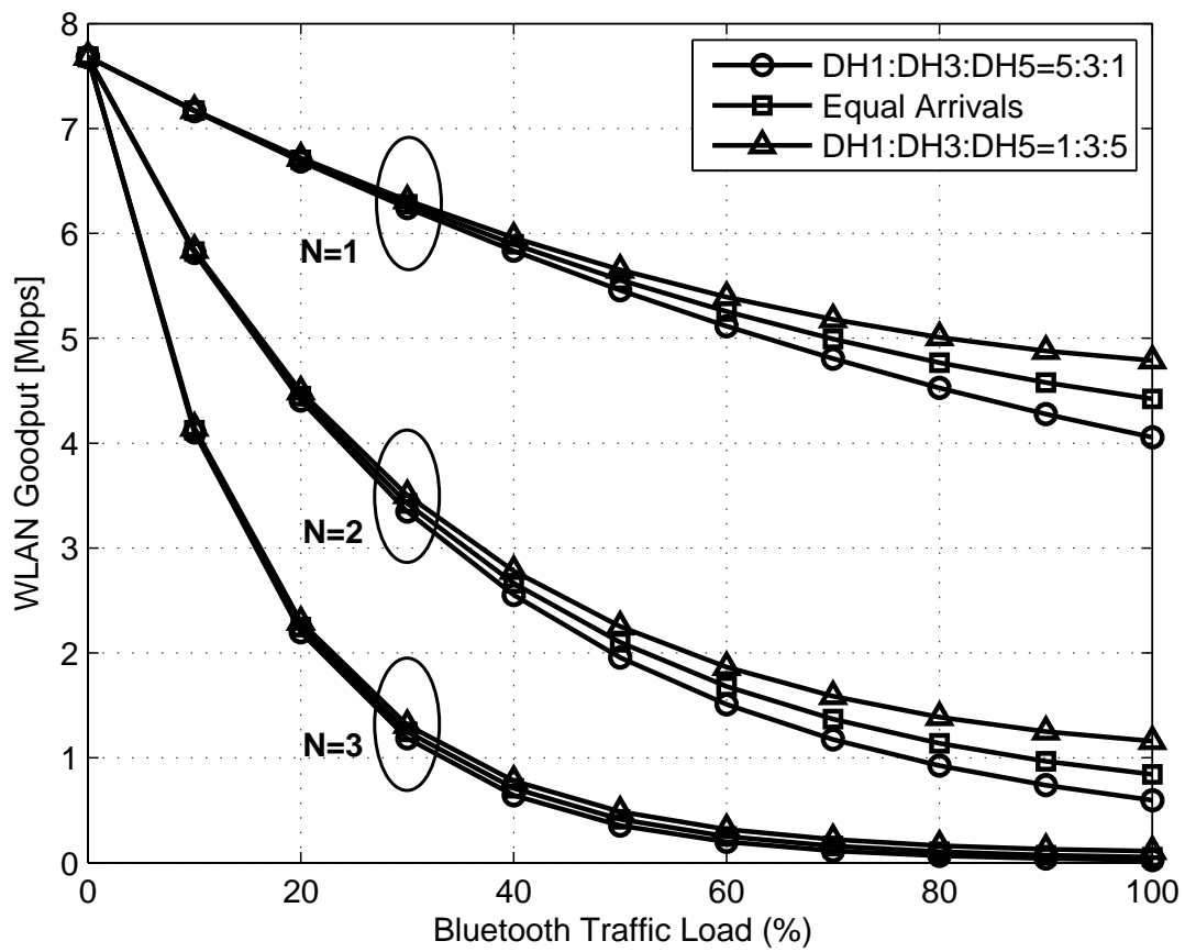
Fig. 12. WLAN Goodput as a function of traffic load in each BT piconet, M = 5 , p = 0.03 , g = 0.1 , WLAN packet size = 1400 bytes ( T_W = 1193 \mu s ), and different arrivals of DH1/3/5.
