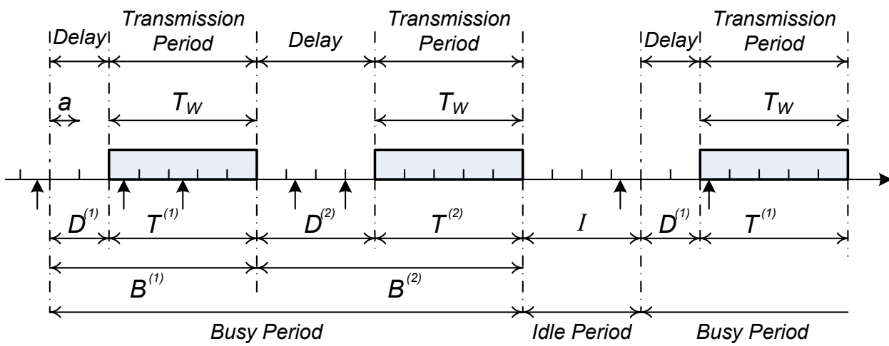
Fig. 7. Channel model for slotted p -persistent CSMA [39]. Small upward arrows indicate the generation of packets by users.
