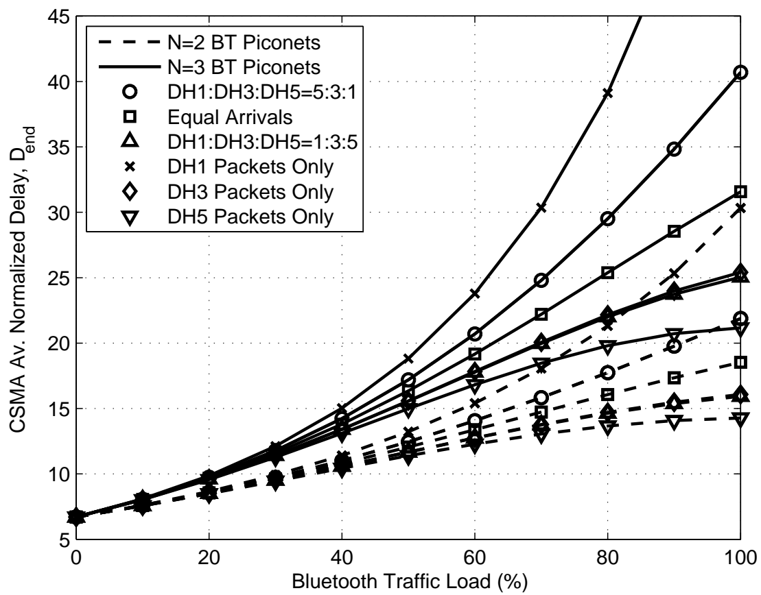
Fig. 15. Average end-to-end CSMA delay as a function of traffic load in each BT piconet, M = 5 , p = 0.03 , g = 0.1 , WLAN packet size = 1400 bytes ( T_W = 1193 \mu s ), and different arrivals of DH1/3/5.
